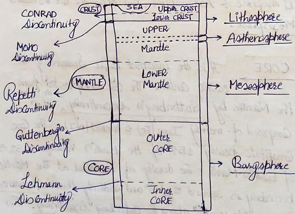
figure → Structure of the Interior of the Earth
